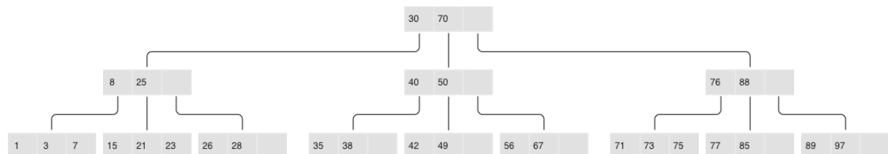
Classical B-tree
